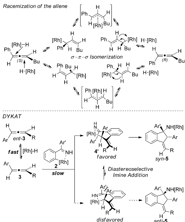
Scheme 4. Mechanistic hypothesis for the allene racemization, DYKAT, and the diastereoselectivity of the addition.
